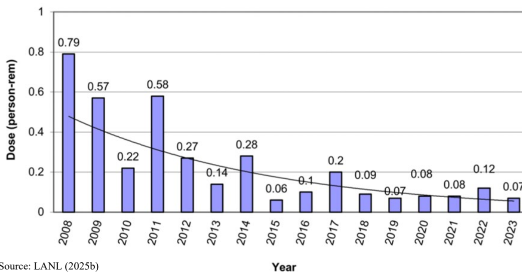
Figure 4.7-2 Trend in Annual Collective Dose to the Population within 50 Miles of LANL
