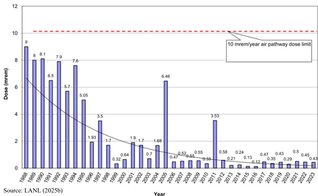
Figure 4.7-1 Trend in Annual MEI Dose at LANL
